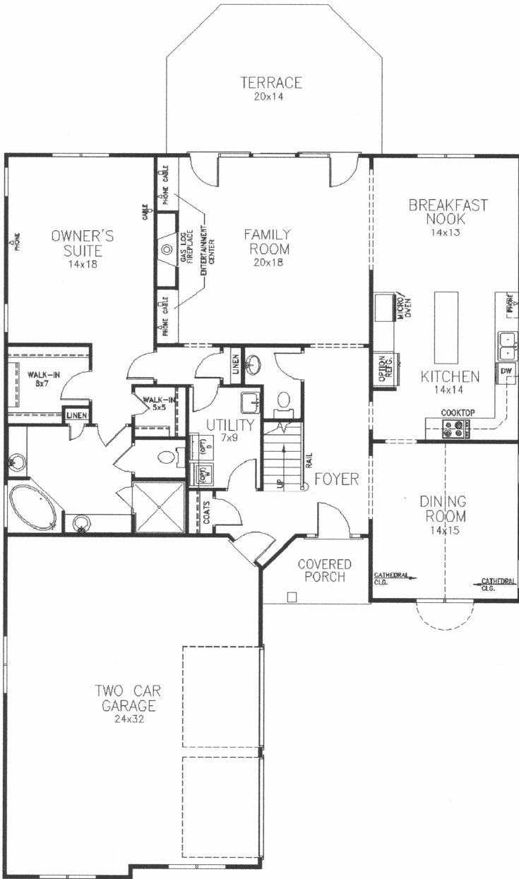
First Floorplan 9' Clg. Hgt.
