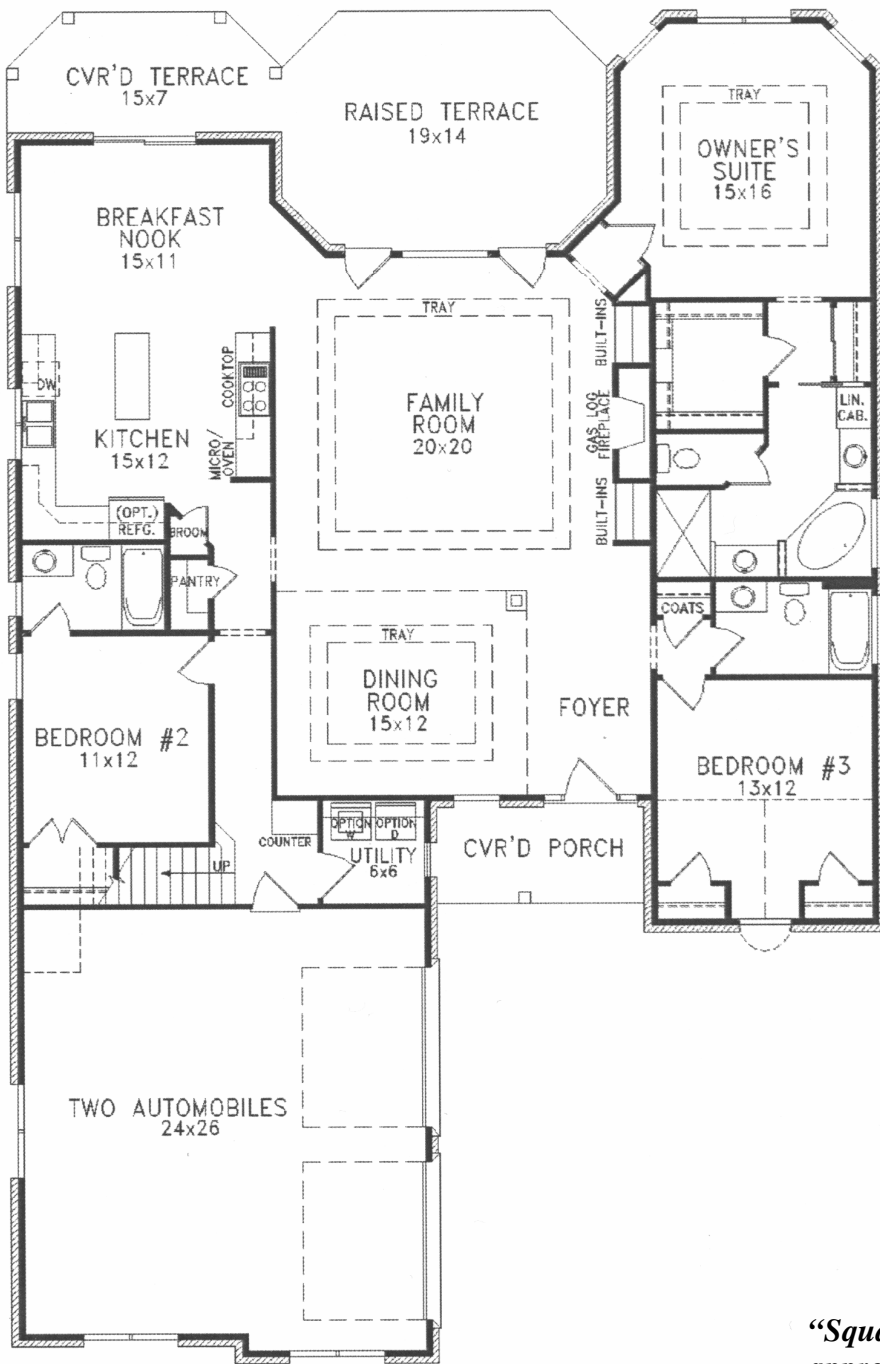
First Floorplan
